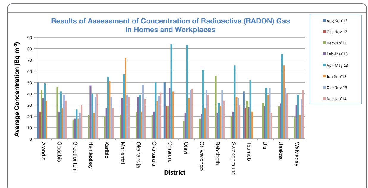
Graph 6: Results of Assessment of Concentration of Radioactive RADON) Gas in Homes and Workplaces
